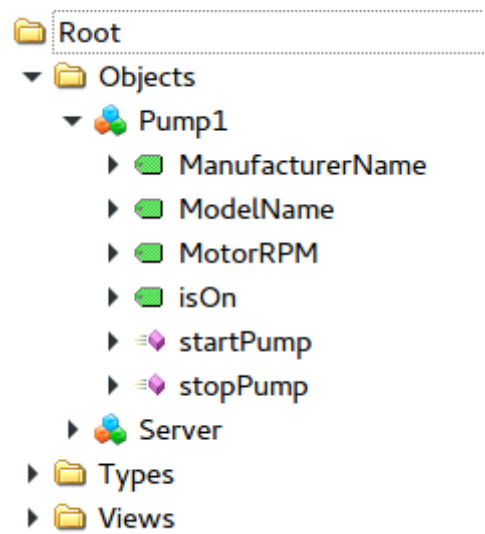
Fig. 10.1: Instantiated Pump Object with inherited children
