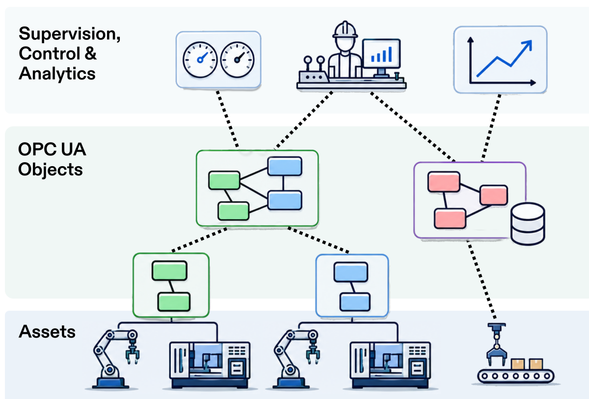
Fig. 2.1: Communication and Object-Oriented Interoperability with OPC UA
