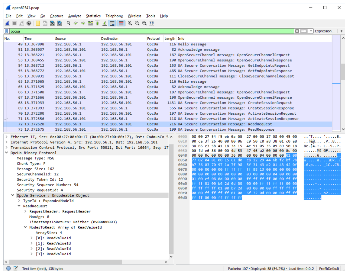
Fig. 2.2: OPC UA conversation displayed in Wireshark
